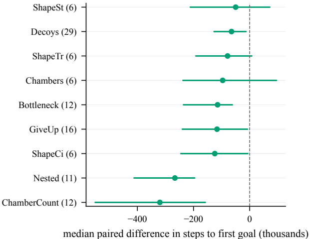
TE + curvature – Go-Explore, by family
