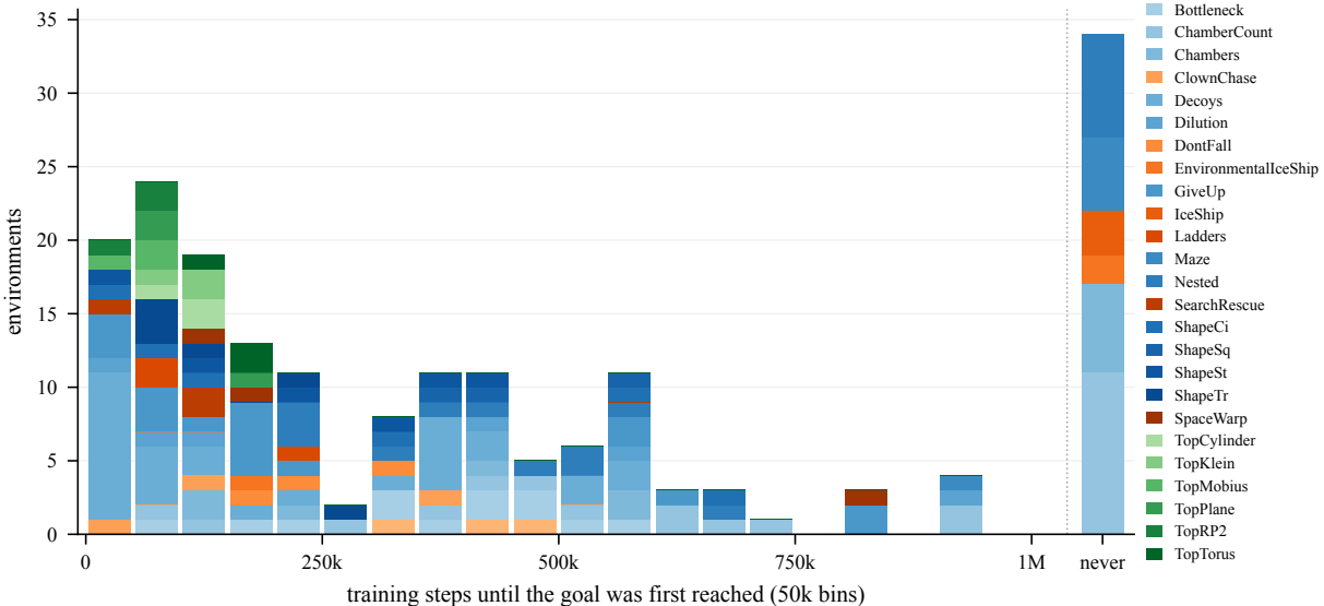
Steps to first goal by family for topoexplore-phase1-animation
