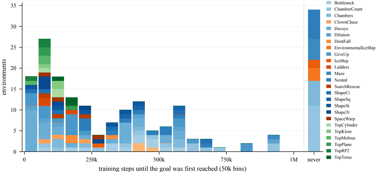
Steps to first goal by family for topoexplore-phase1-none
