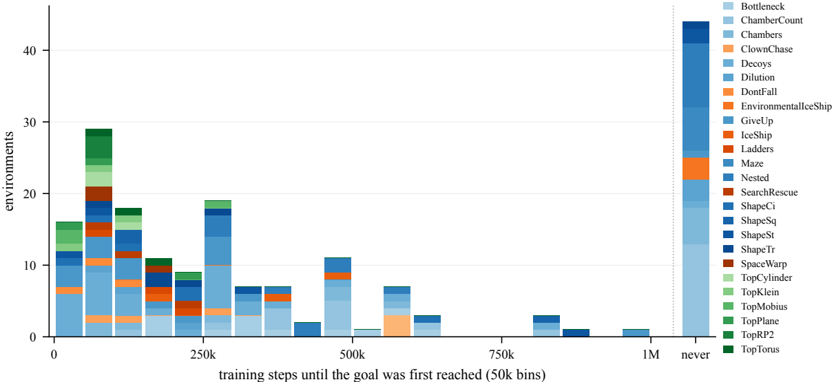
Steps to first goal by family for topoexplore-phase1and2-animation
