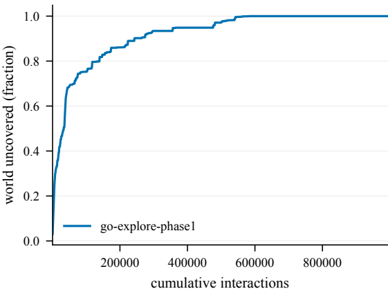
Cumulative coverage -- BankRobber@4001
