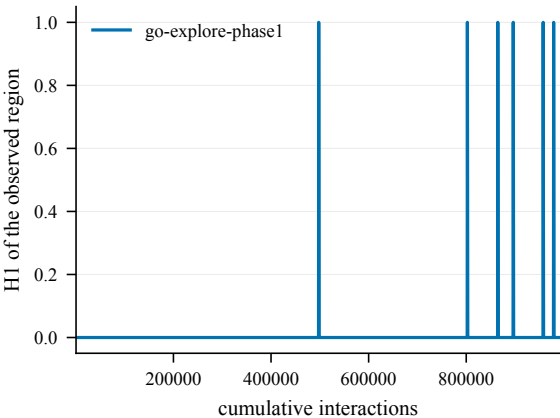
Discovered topology -- BankRobber@4001
