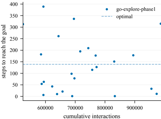
Steps to goal (train) -- BankRobber@4001
