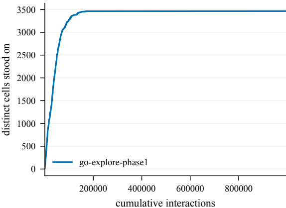
States discovered -- ClownChase@4000
