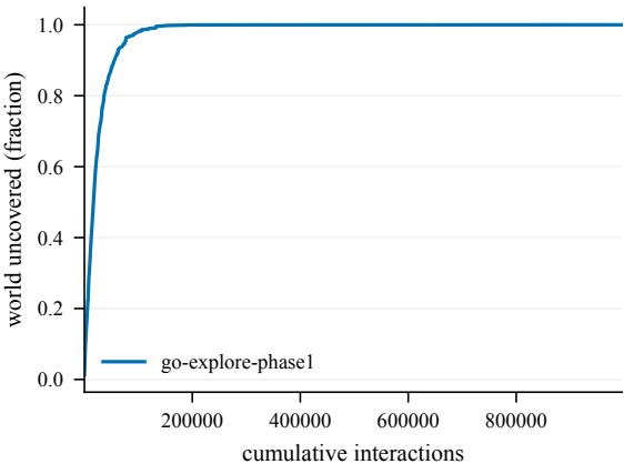
Cumulative coverage -- ClownChase@4001
