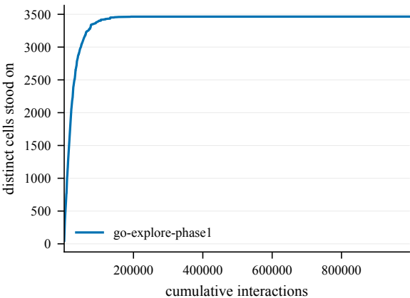
States discovered -- ClownChase@4001
