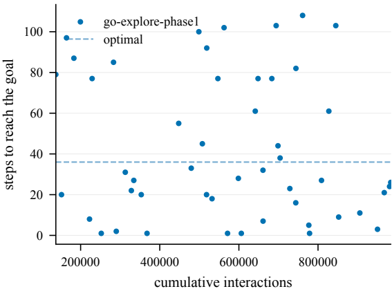
Steps to goal (train) -- ClownChase@4002
