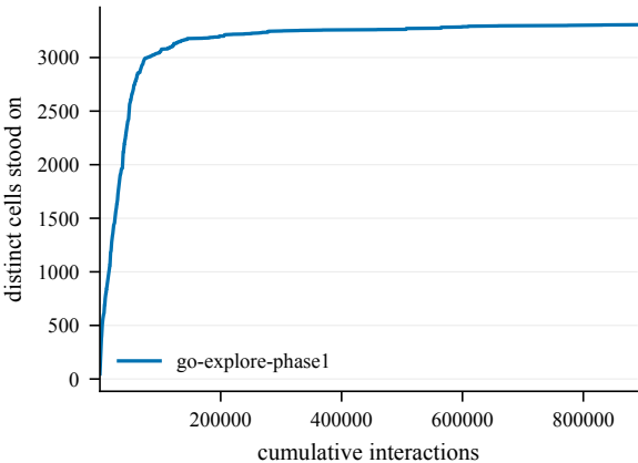
States discovered -- DontFall@4000
