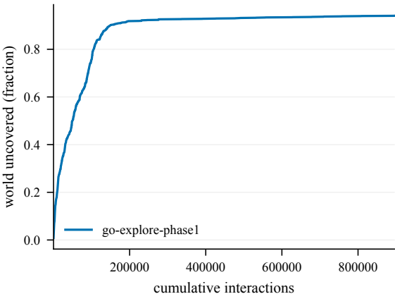
Cumulative coverage -- DontFall@4001
