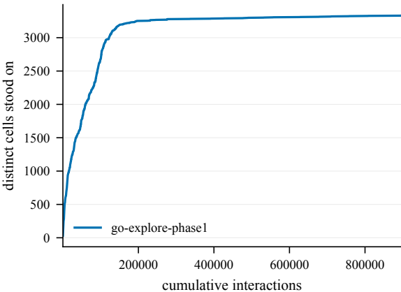
States discovered -- DontFall@4001
