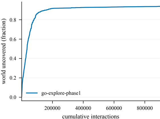
Cumulative coverage -- DontFall@4002
