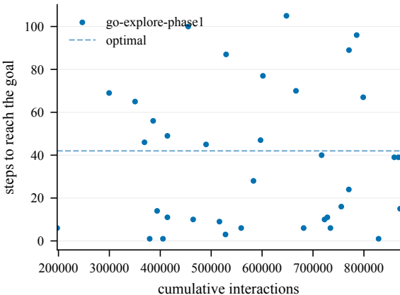
Steps to goal (train) -- DontFall@4002
