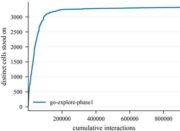
States discovered -- DontFall@4002
