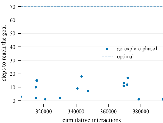
Steps to goal (train) -- EnvironmentalIceShip@4001
