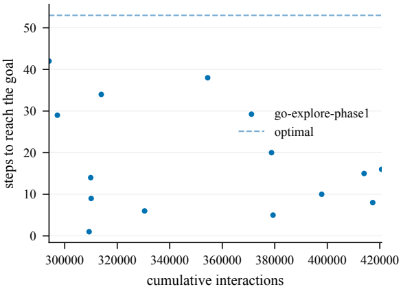
Steps to goal (train) -- EnvironmentalIceShip@4002
