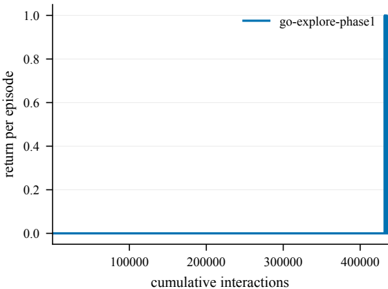
Return -- IceShip@4000
