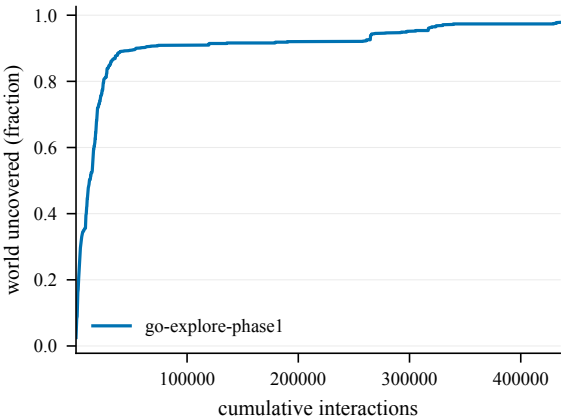
Cumulative coverage -- IceShip@4000
