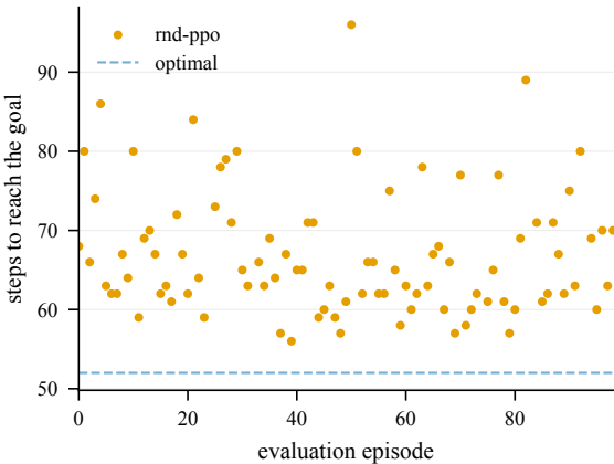
Steps to goal (eval) -- IceShip@4000
