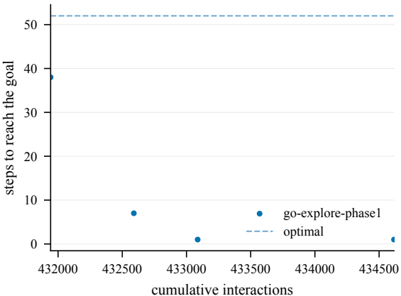
Steps to goal (train) -- IceShip@4000
