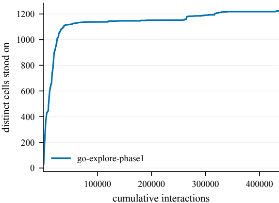
States discovered -- IceShip@4000
