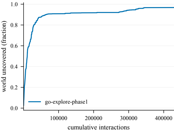
Cumulative coverage -- IceShip@4001
