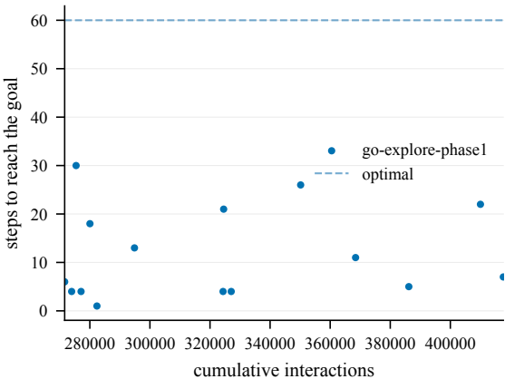
Steps to goal (train) -- IceShip@4001
