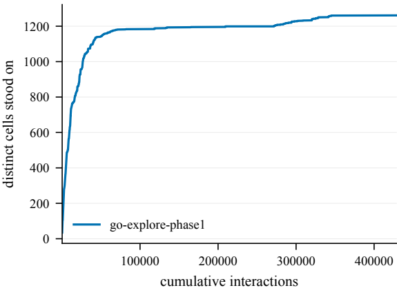
States discovered -- IceShip@4001
