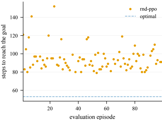
Steps to goal (eval) -- IceShip@4002
