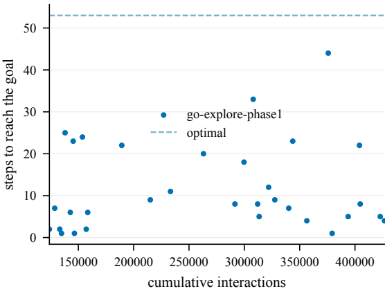
Steps to goal (train) -- IceShip@4002
