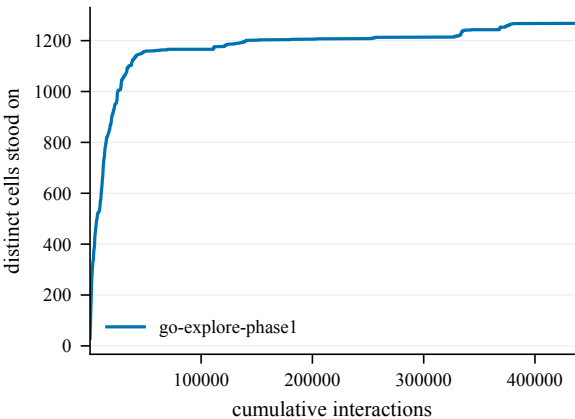
States discovered -- IceShip@4002
