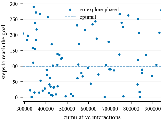
Steps to goal (train) -- Ladders@4000
