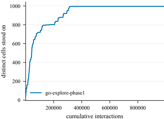
States discovered -- Ladders@4000
