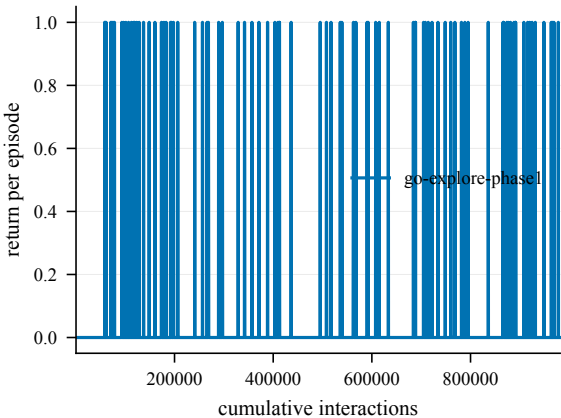
Return -- Ladders@4002
