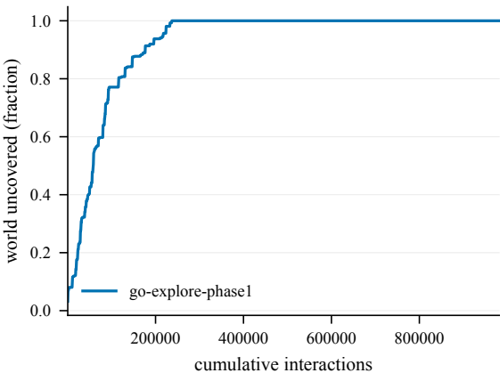
Cumulative coverage -- Ladders@4002
