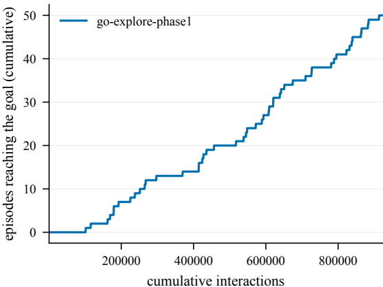
Goal reached -- SearchRescue@4000
