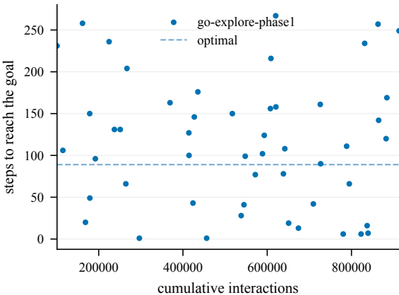
Steps to goal (train) -- SearchRescue@4000
