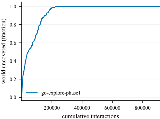
Cumulative coverage -- SearchRescue@4001
