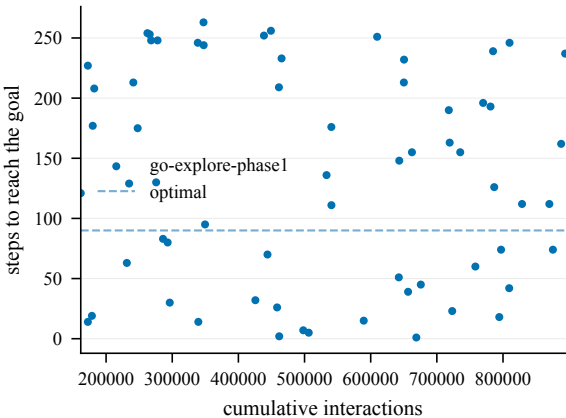
Steps to goal (train) -- SearchRescue@4001
