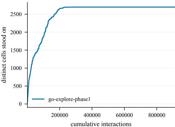
States discovered -- SearchRescue@4001
