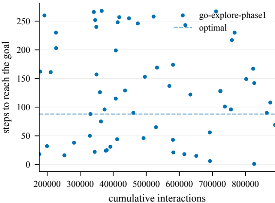
Steps to goal (train) -- SearchRescue@4002
