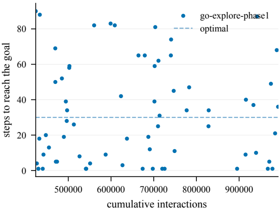
Steps to goal (train) -- SpaceWarp@4000
