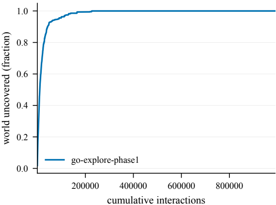
Cumulative coverage -- TopCylinder-50@4000
