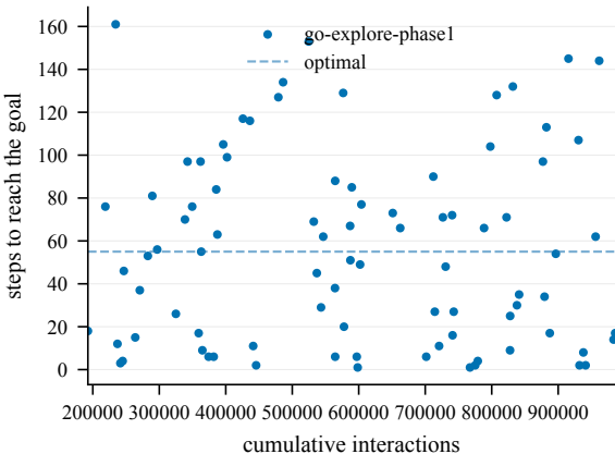
Steps to goal (train) -- TopCylinder-50@4000
