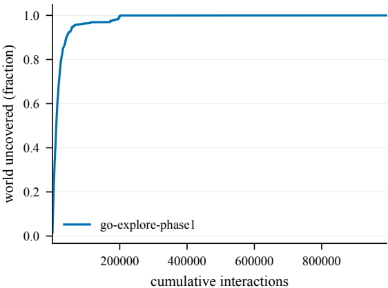
Cumulative coverage -- TopCylinder-50@4001
