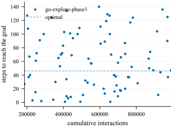
Steps to goal (train) -- TopCylinder-50@4001
