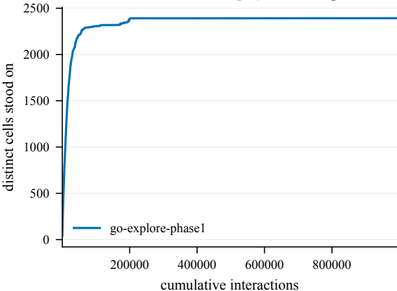
States discovered -- TopCylinder-50@4001
