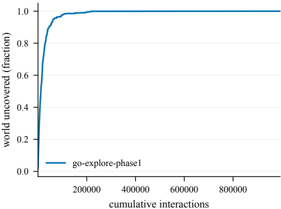
Cumulative coverage -- TopCylinder-50@4002
