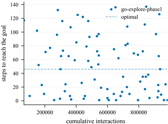
Steps to goal (train) -- TopKlein-50@4001
