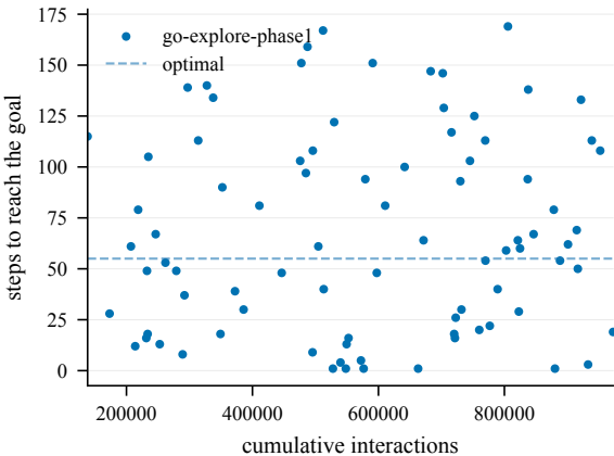
Steps to goal (train) -- TopMobius-50@4000
