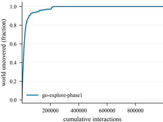
Cumulative coverage -- TopMobius-50@4001
